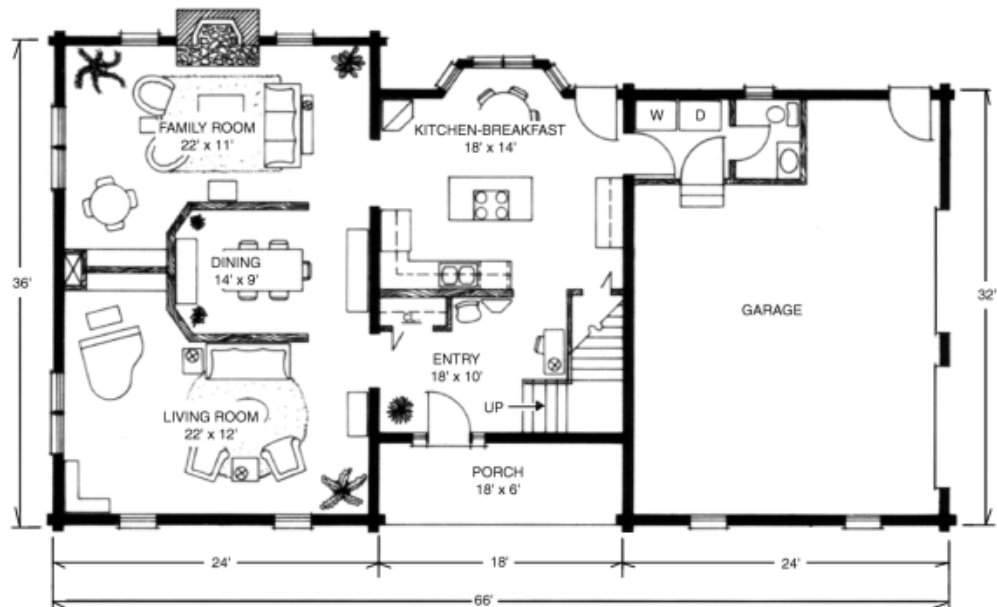
MAIN FLOOR
